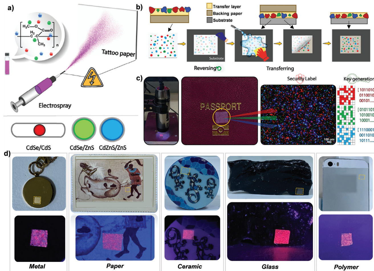
Figure 1. A schematic illustration of the proposed approach for generating tattoo-like multi-color PUFs. a) Electro spraying of fluorescent semiconductor nanocrystals on the tattoo paper. b) Transferring unclonable features via a temporary tattoo paper. c) Demonstration of an application on a passport surface imaging by a handheld fluorescence microscope. Extraction and authentication of multiple PUF keys depending on the emission channels derived from fluorescence images. d) Photographs of PUF labels created on different surfaces such as metal (necklace), paper (antique postage stamp), ceramic (handcrafted brooch), glass (obsidian ore), and polymer (smartphone case).
